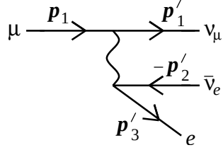
Figure 88.1: Feynman diagram for muon decay. The wavy line is a W propagator.
