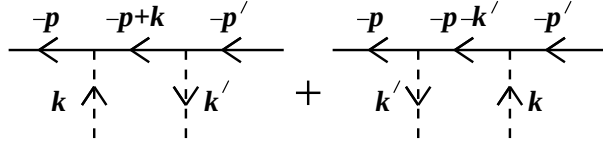
Figure 45.5: Diagrams for e^+\varphi \rightarrow e^+\varphi , corresponding to eq. (45.22).
