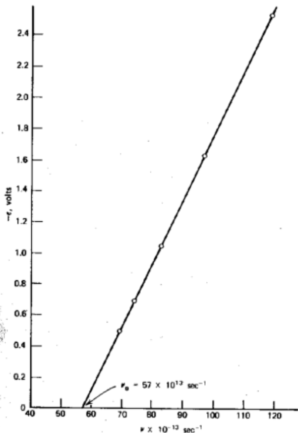
Fig. 1-3. Photoelectric effect data showing a plot of retarding potential necessary to stop electron flow from a metal (lithium), or equivalently, electron kinetic energy, as a function of frequency of the incident light. The slope of the line is h/e .
