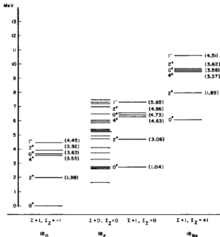
Fig. 26-3. The level schemes for nuclei with A = 18 . The I = 1 levels for ^{18}\text{O} ( I_s = -1 ), ^{18}\text{F} ( I_s = 0 ), and ^{18}\text{Ne} ( I_s = 1 ) show a remarkable correspondence. The I = 0 levels for ^{18}\text{F} are also sketched in. (Data taken from F. Ajzenberg-Selove, Nuclear Physics A190 , 1 (1972).)
