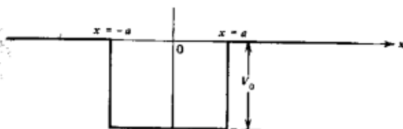
Fig. 5-2. The potential well.
