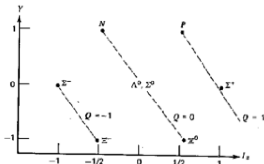
Fig. 26-8. Octet pattern for spin 1/2^+ baryons. The diagonal lines are lines of constant charge Q .
