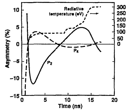
FIG. 115. With a constant power ratio (35% inner cone, 65% outer cone), NIF targets exhibit time-varying asymmetry in the P_2 and P_4 Legendre moments of flux. In detailed 2-D calculations, ignition capsules with this degree of time variation ignite and give yields near those seen for spherical implosions with uniform radiation drive. This degree of temporal variation in flux uniformity is near the maximum tolerable and would be reduced by "beam phasing" in which the power fraction in the inner and outer cones is varied in time.
