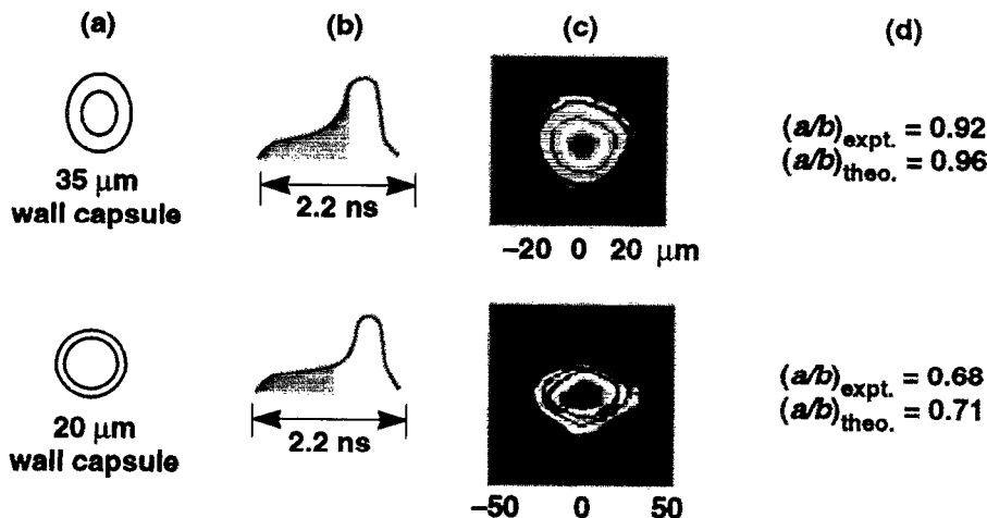
FIG. 81. Data from ps22 using the variation in implosion time of capsules with different wall thickness: (a) initial capsule configuration; (b) shaded portion of the drive represents the effective sampling interval for the implosion for the two cases; (c) implosion image data taken orthogonal to the hohlraum axis; and (d) comparison of the measured capsule eccentricity with the calculated value.
