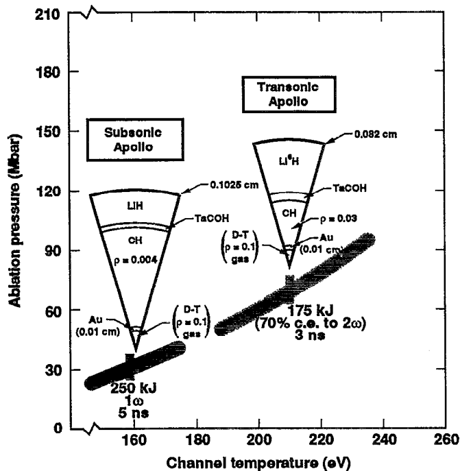
FIG. 26. Calculations in 1979, which predicted ignition for a 20-beam "200 kJ Nova," required high hohlraum coupling efficiency and near 1-D performance of double-shell targets. Both capsules had E_{\text{cap}} = 50 kJ, V(\text{TaCOH}) = 2 \times 10^7 cm/s, V(\text{Au}) = 3 \times 10^7 cm/s. Capsule yields were about 100 kJ.
