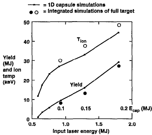
FIG. 114. Scales of the point design ignite above about 700 kJ. For the 1-D capsule simulations, capsule dimensions and times are scaled by s , and the effective laser energy is given by E_{\text{eff}}(\text{MJ}) = 1.35s^3 , where s=1 is the PT design. For the integrated hohlraum and capsule simulations, dimensions and times are proportional to s , and powers are proportional to s^2 .
