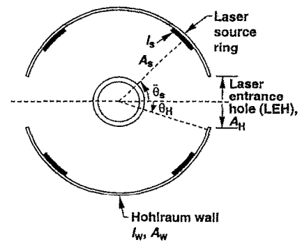
FIG. 63. A simplified spherical hohlraum is used to analyze hohlraum symmetry.
