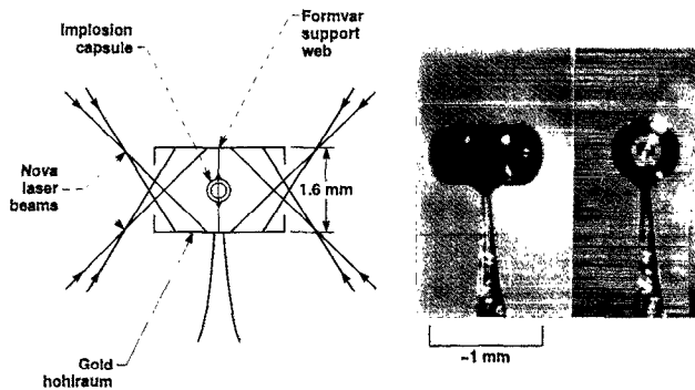
FIG. 10. Nova implosion target, illustrating beam geometry. Five Nova beams irradiate each side of the hohlraum. The beams are uniformly distributed around the rim of a 100^\circ cone.
