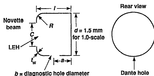
FIG. 32. Half-Cairn targets for Novette scaling experiments. Dimensions: d =outside diameter of cylinder= 1500\text{ }\mu\text{m} for 1.0 scale; l =length of cylinder= (5/6)d ; a =distance from back wall to center of Dante hole= (13/30)d ; b =diameter of Dante hole= (4/15)d ; c =LEH diameter= 0.5d ; t_w =wall thickness; R =radius of front corner= 0.25d ; g =back corner angle= 90 \pm 2^\circ .
