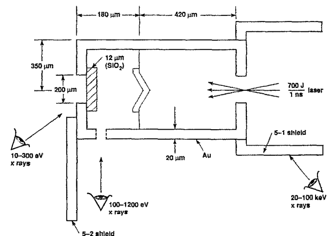
FIG. 16. Target setup for a coupling experiment on the Argus laser. We measured the coupling of radiation (burnthrough) and superthermals (preheat) to a 12\ \mu\text{m} slab of glass ( 100\times -like target) in a 100\times -like environment (half-Cairn).
