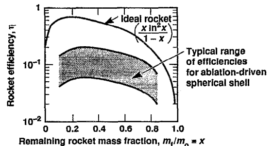
FIG. 5. Subsonic ablation follows an isothermal rocket equation. Radiation-driven implosions typically have an efficiency of 15%–20%. Direct-drive efficiency depends on laser wavelength and illumination geometry, but is typically 5%–10%; x = m_f/m_0 is the ratio of the final shell mass m_f to the initial mass m_0 .
