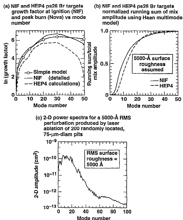
FIG. 48. Growth-factor spectrum for ps26 brominated targets compares well with NIF targets.
