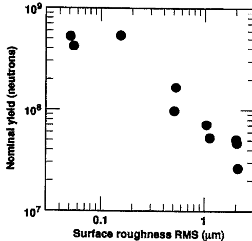
FIG. 50. Quantitative studies of implosions with large RT growth factors are now possible. For the HEP-4 capsules, surface roughness is imposed by precision laser ablation during fabrication. Precision Nova operation has dramatically reduced shot-to-shot yield variations, making these measurements possible.
