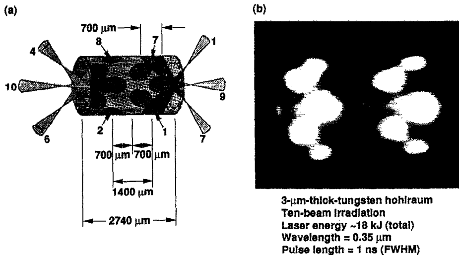
FIG. 67. X-ray imaging of thin-wall hohlraums shows high absorption and little spot motion or beam spreading for 1 ns pulses (1986 Nova data): (a) relative beam pointing for a scale-1.0 hohlraum (ten beams); (b) relative beam spot positions, as imaged with a \sim 50 \mu\text{m} resolution pinhole camera.
