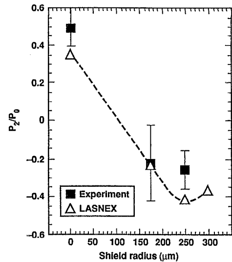
FIG. 79. The effect of LEH shields on Nova hohlraums can be modeled quantitatively.
