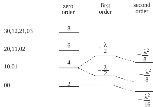
Figure 1: Energy levels for coupled oscillators.
