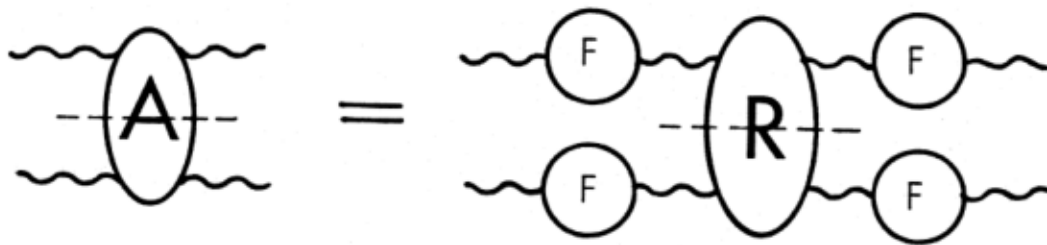
Fig. 29. Relation between discontinuity A and the Toller-normalized 4-Reggeon ring discontinuity. The R-notation is that of Ref. 7. XBL 779-2318
