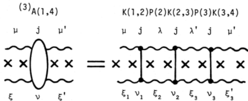
Fig. 24. The 3-particle/cluster contribution to the 4-Reggeon amplitude, in both energy-plane and j -plane.
