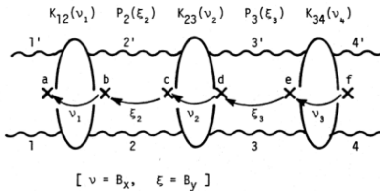
Fig. 22. The 3-particle or 3-cluster contribution to the 4-Reggeon amplitude.
