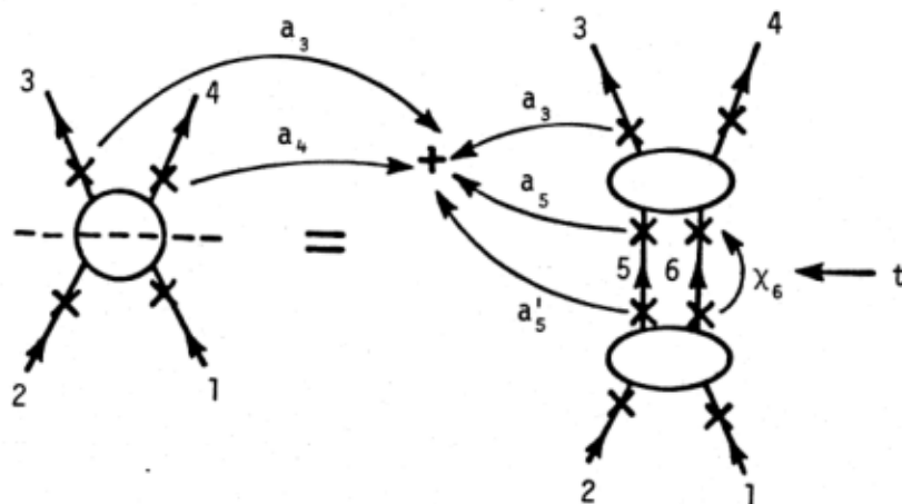
Fig. 7. Elastic unitarity; \chi_6 is the Misheloff rotation for particle 6.
