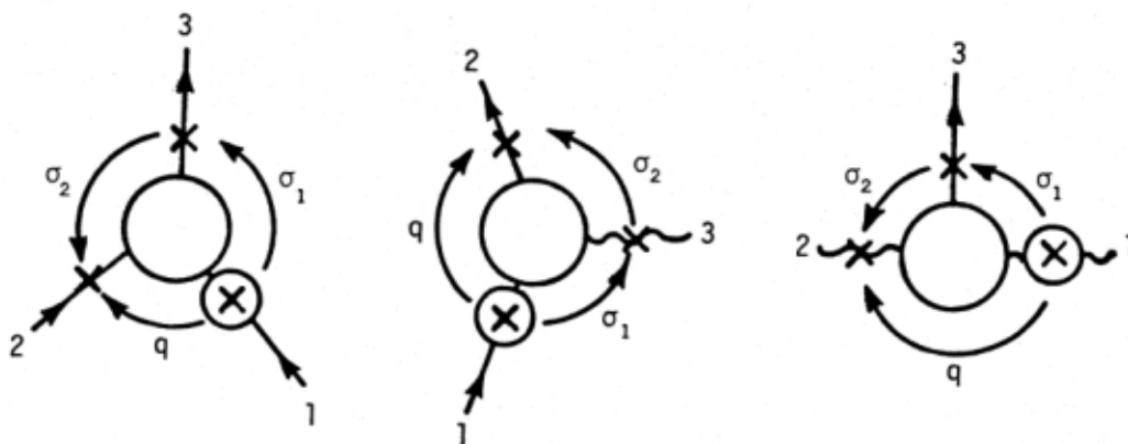
Fig. 6. The standard Toller vertex in no-Regge, single-Regge, and double-Regge configurations.
