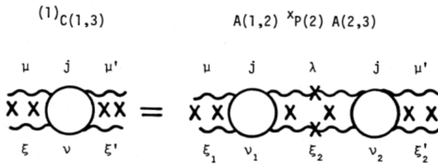
Fig. 36. The C^{(1)} cylinder term with exact kinematics.
