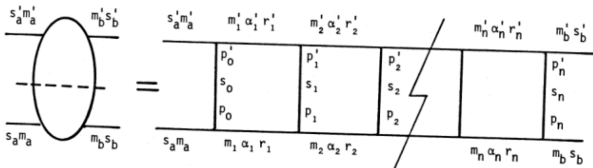
Fig. 9. Spin and helicity labeling for multiperipheral unitarity product. Upper variables are primed versions of lower variables.
