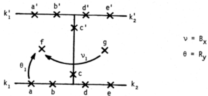
Fig. 13. Central level frames f and g added to the rung.
