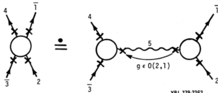
Fig. 4. A Regge pole contribution to the 4-point function.
