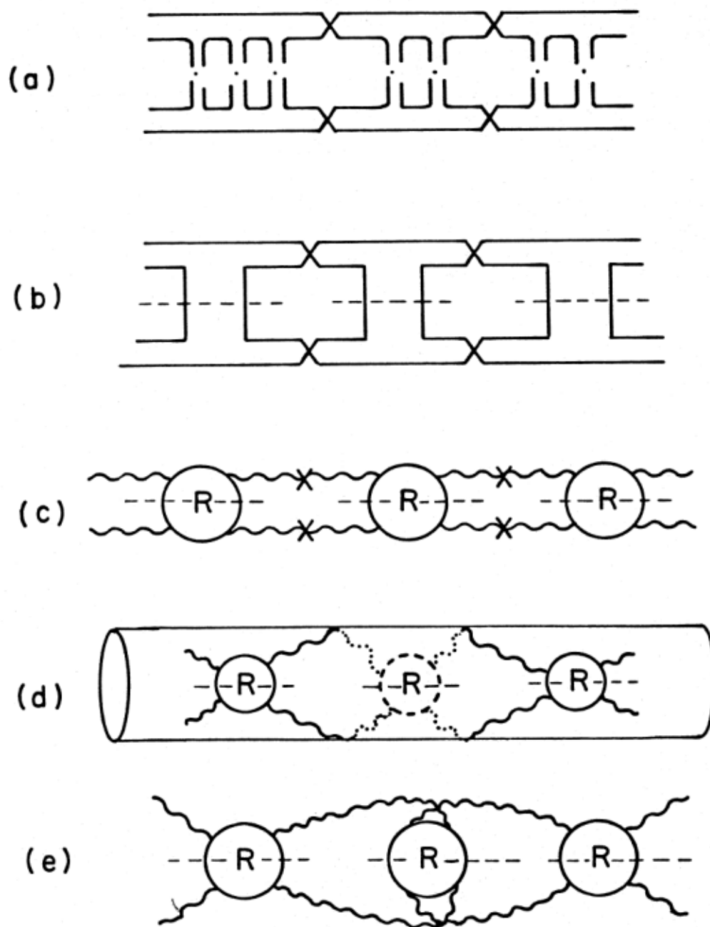
Fig. 33. The two twist-pair contribution to the cylinder in various notations (see text). XBL 779-2314
