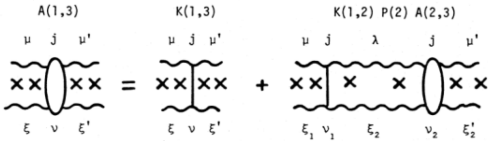
Fig. 25. The bootstrap equation in both energy- and j -planes.
