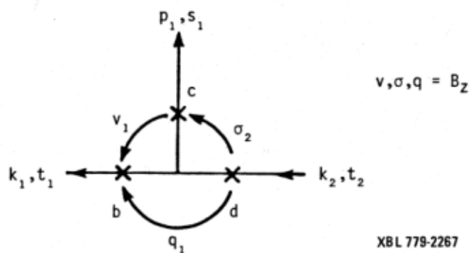
Fig. 10. The BCP frame triad for a production vertex.
