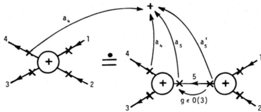
Fig. 3. A particle pole term contained in the 4-point function.
