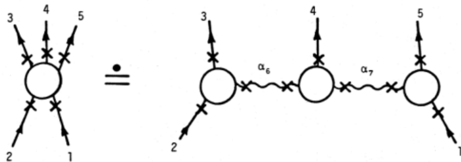
Fig. 5. A double-Regge contribution to the 5-point function.
