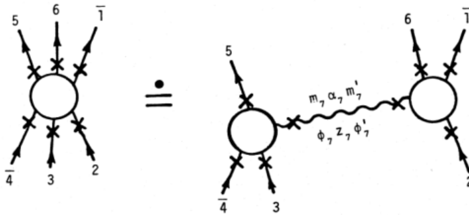
Fig. 2. A Regge pole contribution to the 6-point function.
