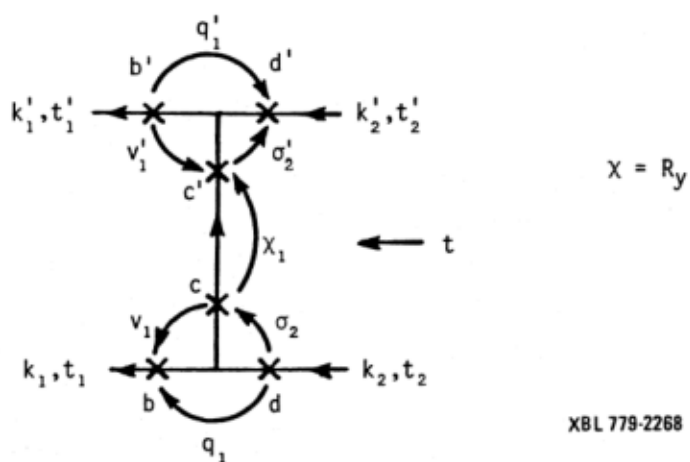
Fig. 11. Two vertices combined to make one rung.
