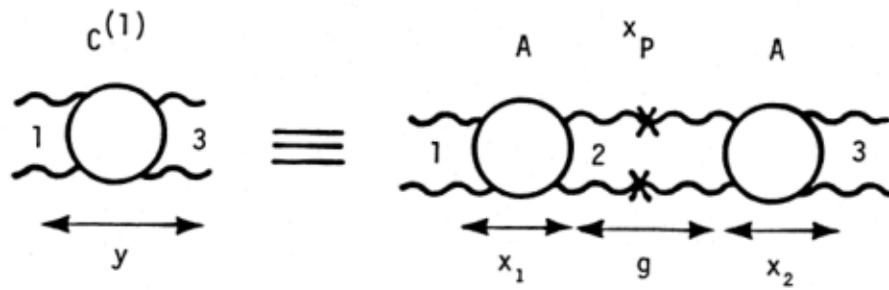
Fig. 35. The C^{(1)} cylinder term in the rapidity model.
