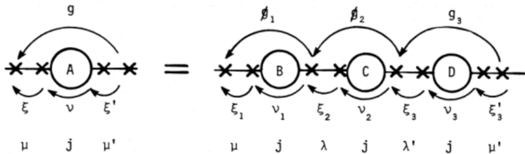
Fig. 23. Functions B, C, D are convoluted to give function A. The variables on the bottom line are conjugate to the boost parameters as shown. The diagonal variable j is angular momentum, variables \mu and \lambda are helicities.
