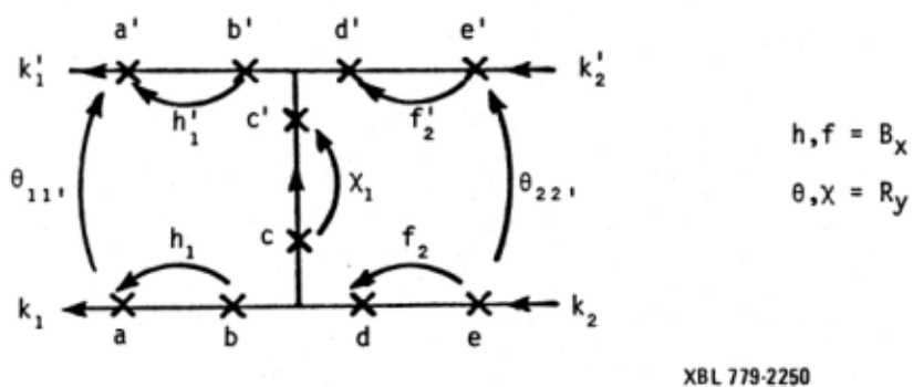
Fig. 12. Four new frames added to the rung.
