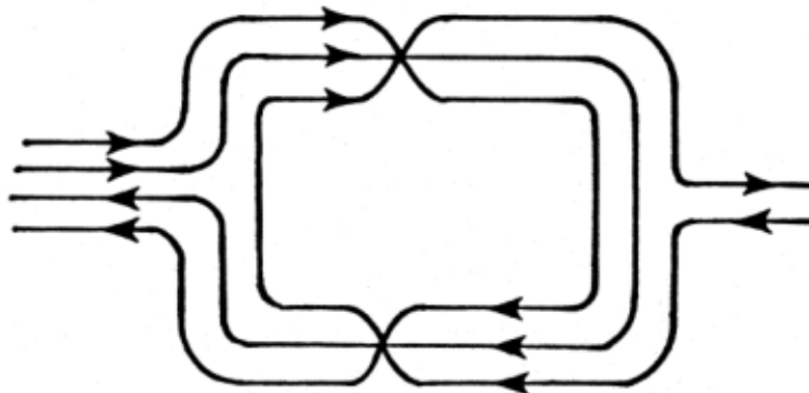
Fig. 39. Quark line structure of twisted Reggeon loop coupling meson to baryonium. Since loop Reggeons are fermions, \epsilon -factors in propagator are set to one-half.
