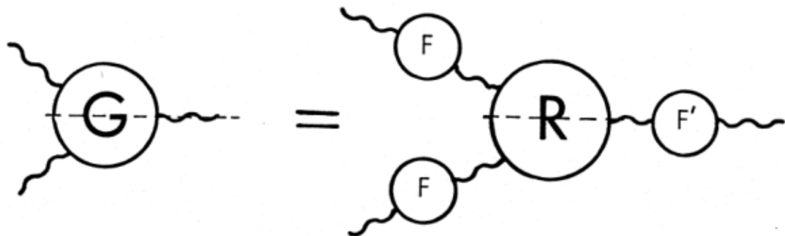
Fig. 30. Relation between the cut vertex G and the Toller-normalized ring function R. XBL 779-2319
