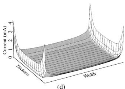
FIGURE 6.14(d). Current distribution over the cross section of a 1.4 mil \times 15 mil land at 1 GHz.
