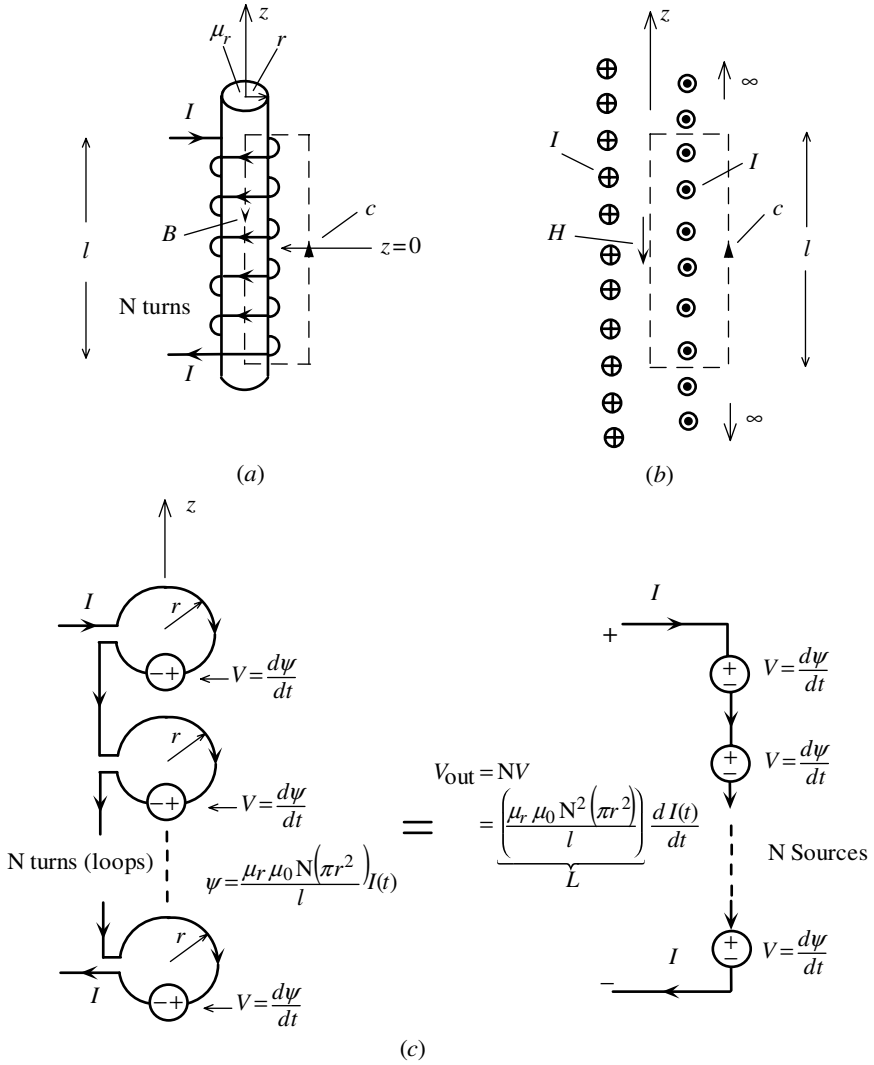
FIGURE 4.7. Solenoid.
