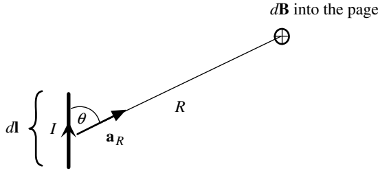
FIGURE 2.6. Biot–Savart law.
