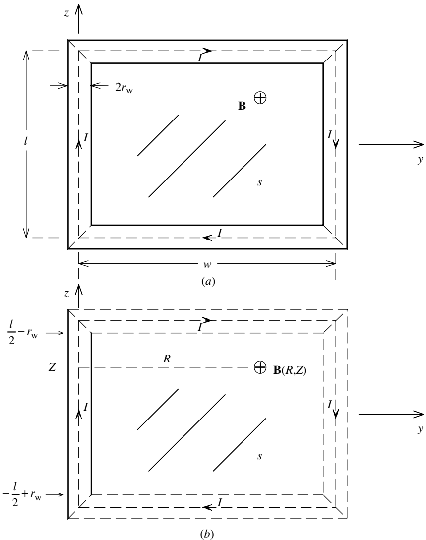
FIGURE 4.3. Rectangular loop.
