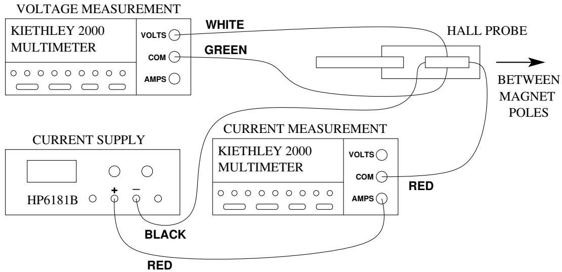
Figure 2: Schematic of Hall Effect experiment. The blade of the probe should be slipped between the magnet pole pieces so that the sensing element is centered.
