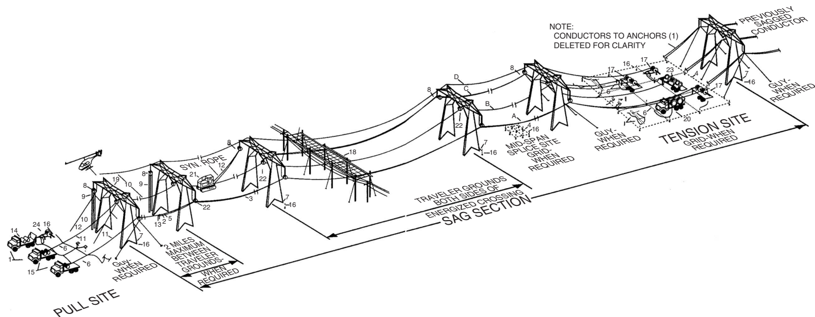
FIGURE 14.10 Tension stringing equipment setup.
