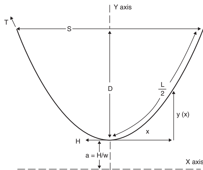
FIGURE 14.1 The catenary curve for level spans.
