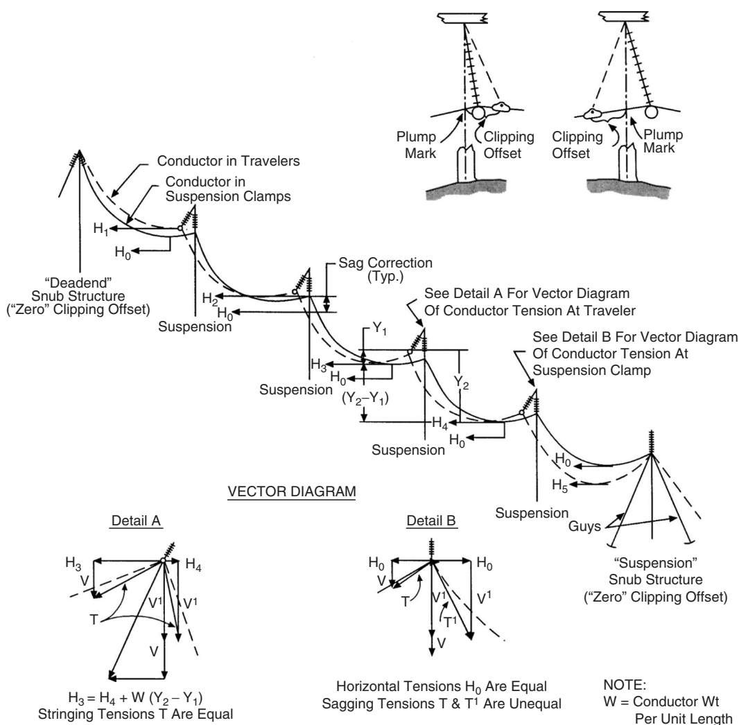
FIGURE 14.13 Clipping offset illustration.
