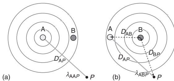
FIGURE 13.10 Flux linkage of (a) conductor A at point P and (b) conductor B on conductor A at point P . Single-phase system.
