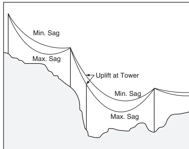
FIGURE 14.9 Conductor uplift.
