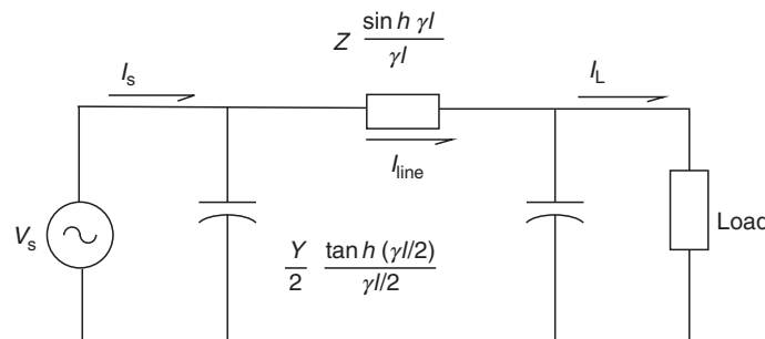
FIGURE 13.3 Equivalent circuit of a long-length transmission line. Z = zl = equivalent total series impedance ( \Omega ), Y = yl = equivalent total shunt admittance (S), z = series impedance per unit length ( \Omega/m ), y = shunt admittance per unit length (S/m), \gamma = \sqrt{ZY} = propagation constant.
