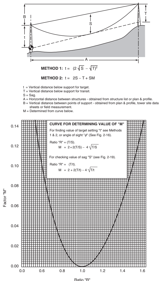
FIGURE 14.17 Conductor sagging by calculated target method.
