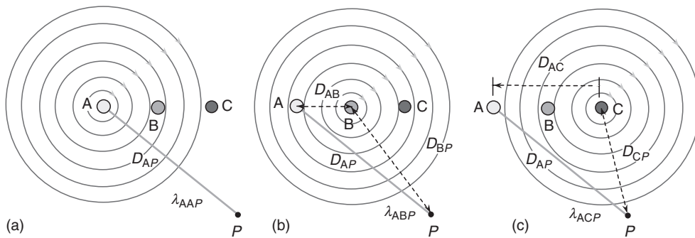
FIGURE 13.12 Flux linkage of (a) conductor A at point P, (b) conductor B on conductor A at point P, and (c) conductor C on conductor A at point P. Three-phase system.
