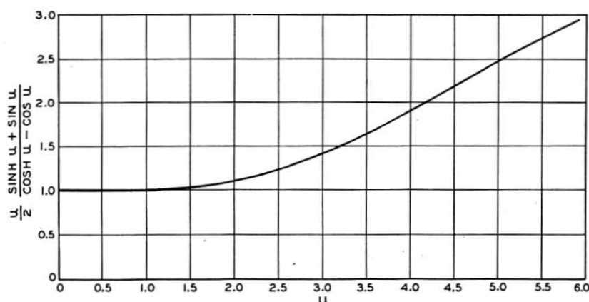
Fig. 5—The skin effect in cylindrical shells. The curve represents the ratio of the a-c. resistance of a typical shell to its d-c. resistance.
