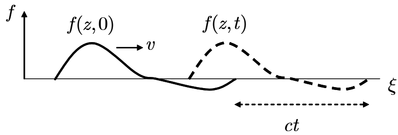
Figure 3.1: The wave tal , in a lossless medium, propagates at velocity tal to the right without changing shape
