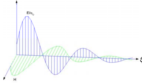
Figure 3.3: Cuidado!!! están normalizada a \eta_0 positive \xi traveling fields of a uniform plane in dissipative medium
