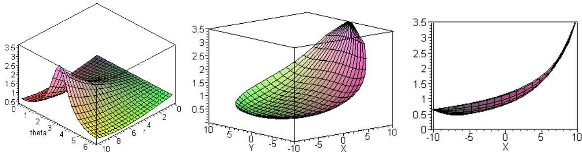
|J_z| Distribution in left round wire for a = 10 , \delta = 5 and \xi_1 = -1.00
