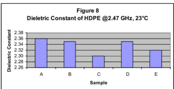
Figure 8: Dielectric Constant of HDPE @ 2.47 GHz, 23°C
