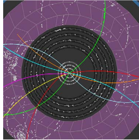
Particle Tracks (B field out of paper) Fig N.2
