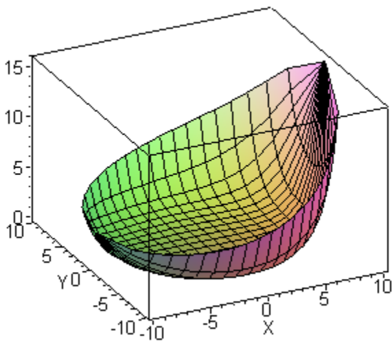
|J_z| Distribution in left round wire for a = 10 , \delta = 1 and \xi_1 = -1.00
