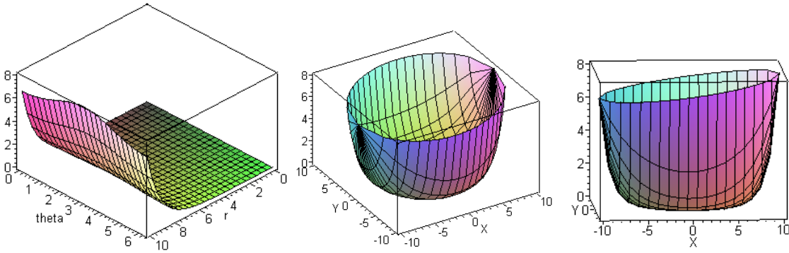
|J_z| Distribution in left round wire for a = 10 , \delta = 1 and \xi_1 = -3.00
