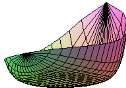
|J_z| Distribution in left round wire for a = 10 , \delta = 1 and \xi_1 = -1.00
